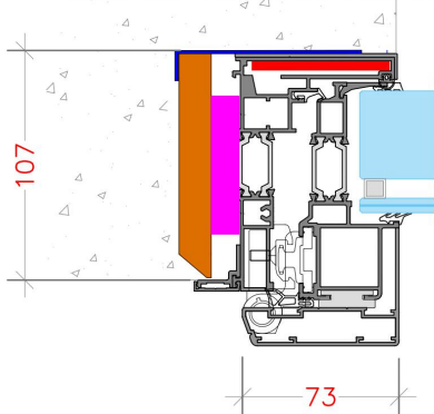
NODO LATERALE— LATO CERNIERA Lateral section— hinge side
